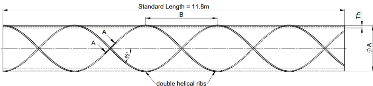
Figure 4. VSL STAY PIPE drawing dimensions.
