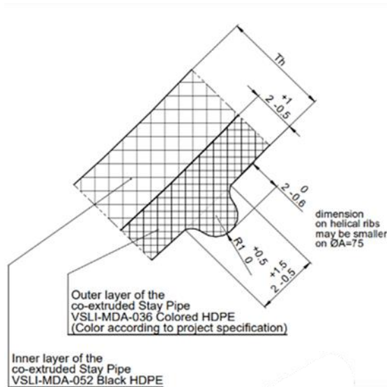
Figure 2. Structure of Coloured stay pipe
